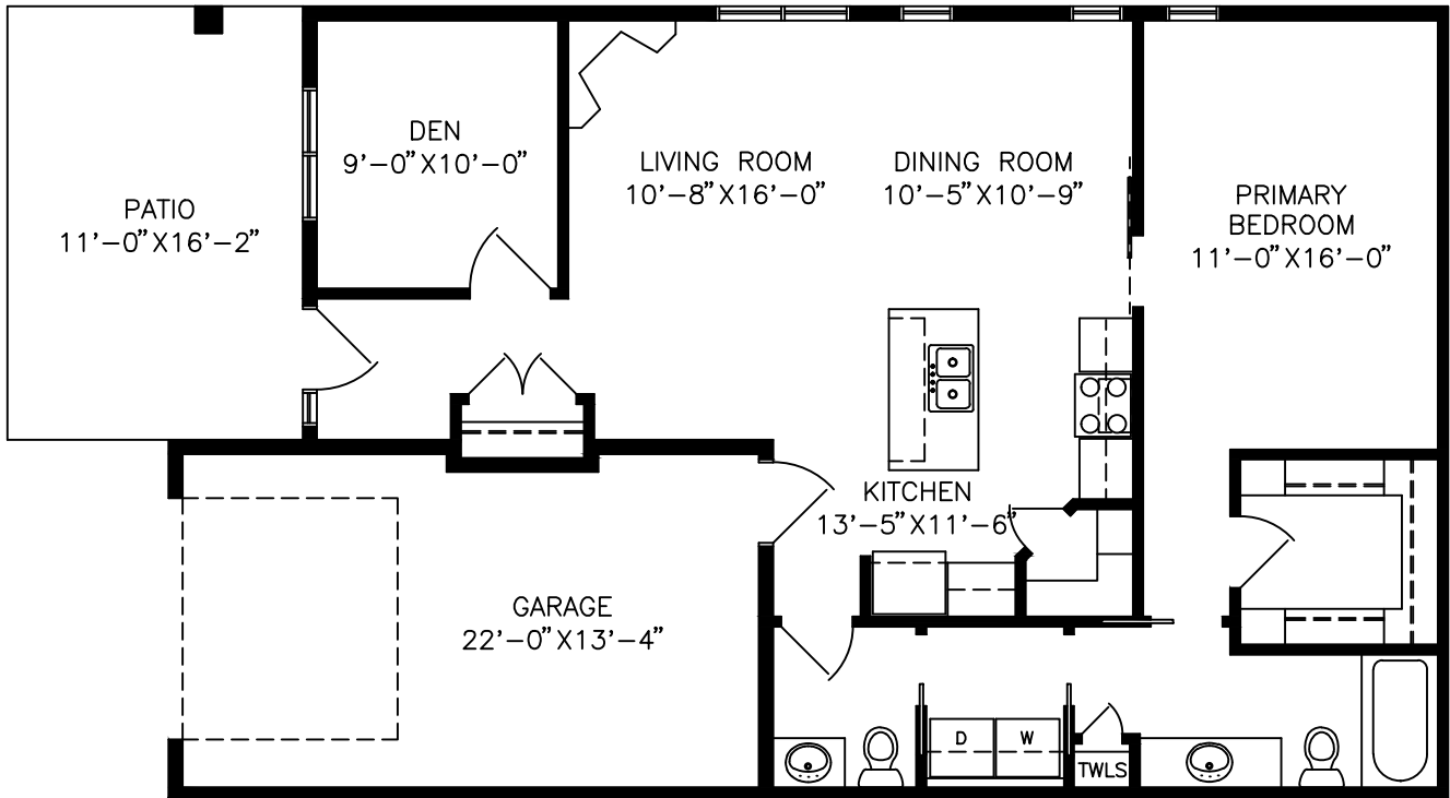
MAIN FLOOR PLAN - UNIT A 1039 SF
